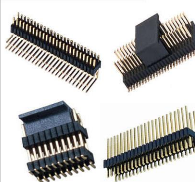
3.96mm pitch pin header
