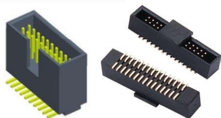
2.54mm pitch Box Header IDC type
