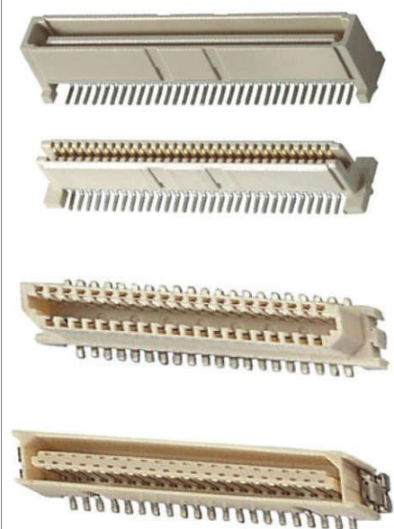
1.25mm pitch BTB connector
