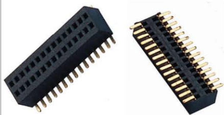
1.0mm pitch female header
