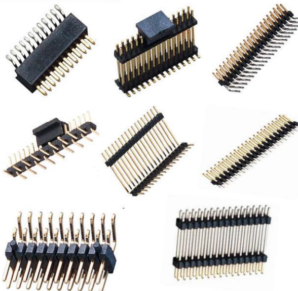
2.0mm pitch pin header
