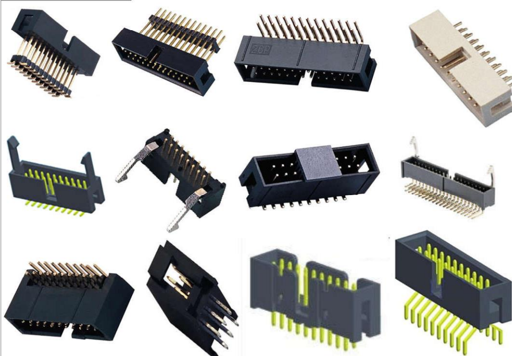
2.54mm pitch Box Header
