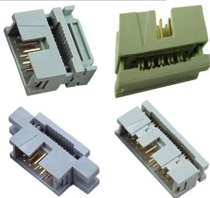
2.54mm pitch Ejector Header IDC type
