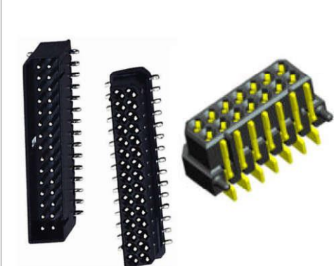
1.25mm pitch BTB connector
