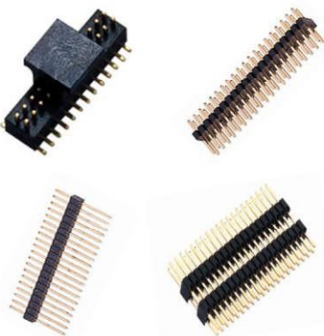
2.2mm pitch pin header
