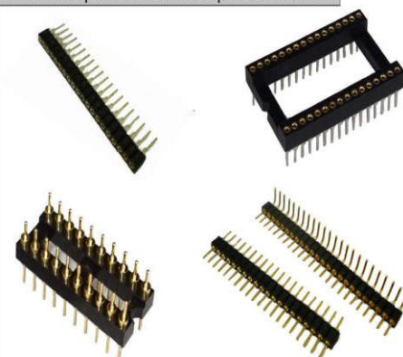
2.54mm pitch machined pin connector
