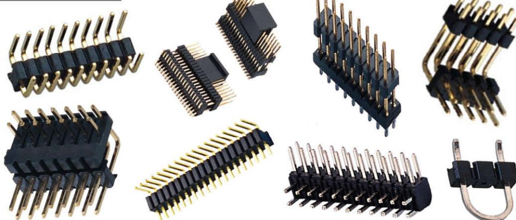
2.54mm pitch pin header
